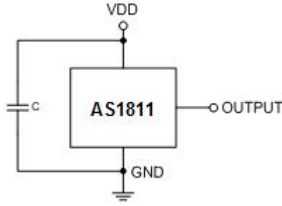
Figure 1, Typical Application Circuit of AS1811
