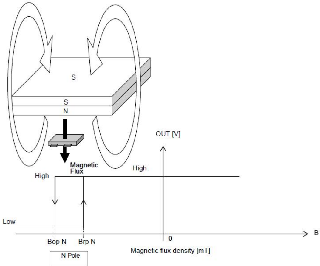
Fig 4, Magnetic Operation Characteristic of AS1811
