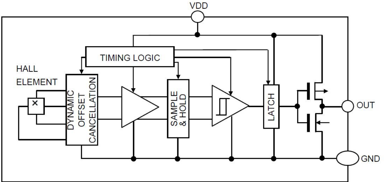
Figure 3, Block Diagram of AS1811
